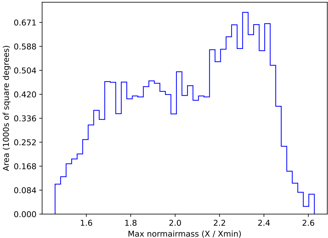
roll_pause_mjdp270_v3.4_10yrs WFD r band: Max normairmass
