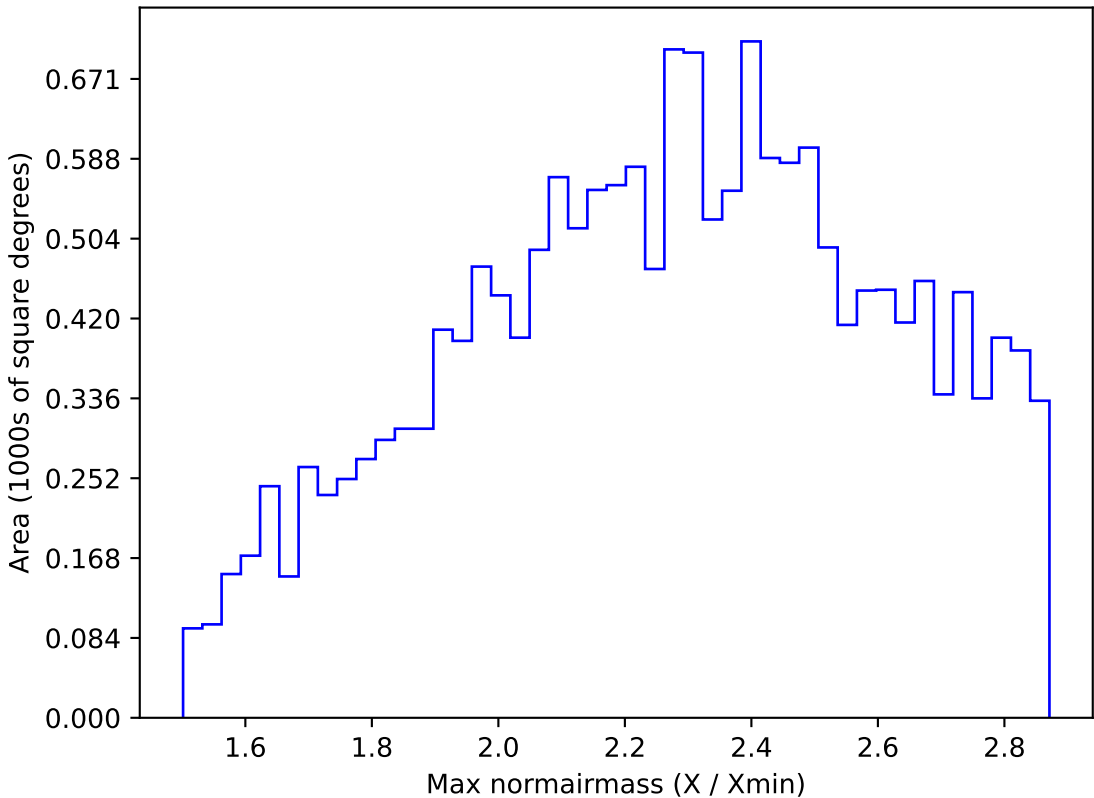
roll_pause_mjdp270_v3.4_10yrs WFD i band: Max normairmass
