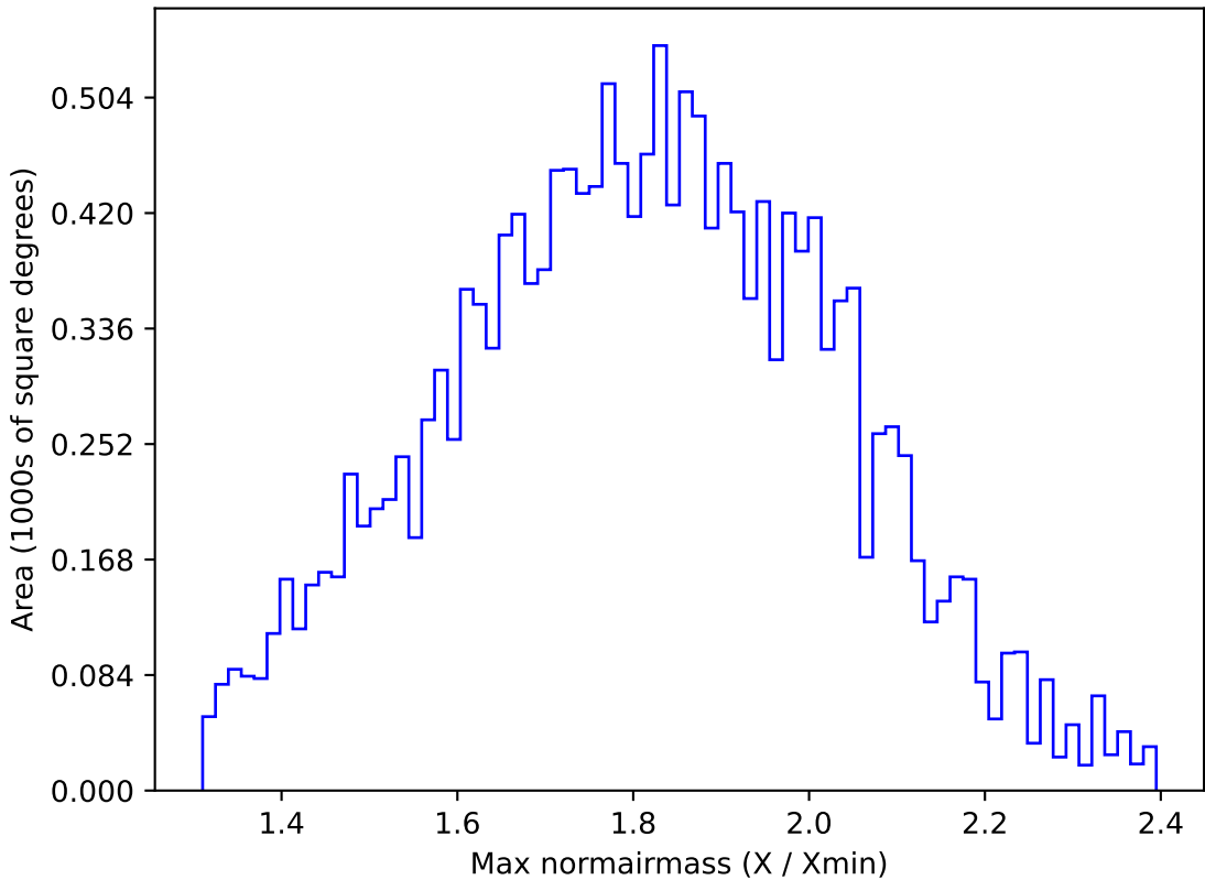
roll_pause_mjdp270_v3.4_10yrs WFD g band: Max normairmass
