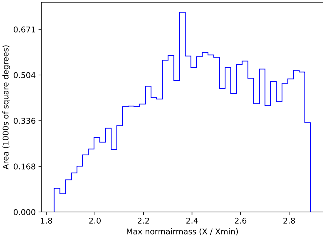
roll_pause_mjdp270_v3.4_10yrs WFD all bands: Max normairmass
