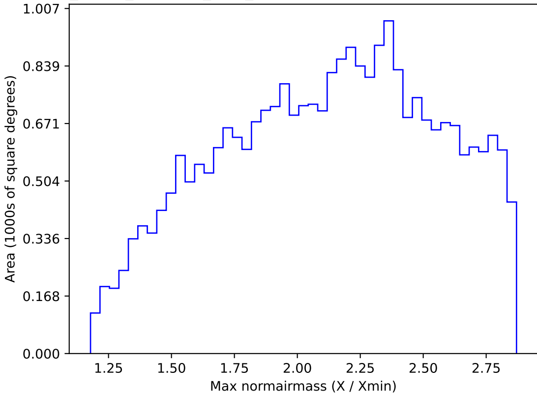
roll_pause_mjdp270_v3.4_10yrs All sky z band: Max normairmass
