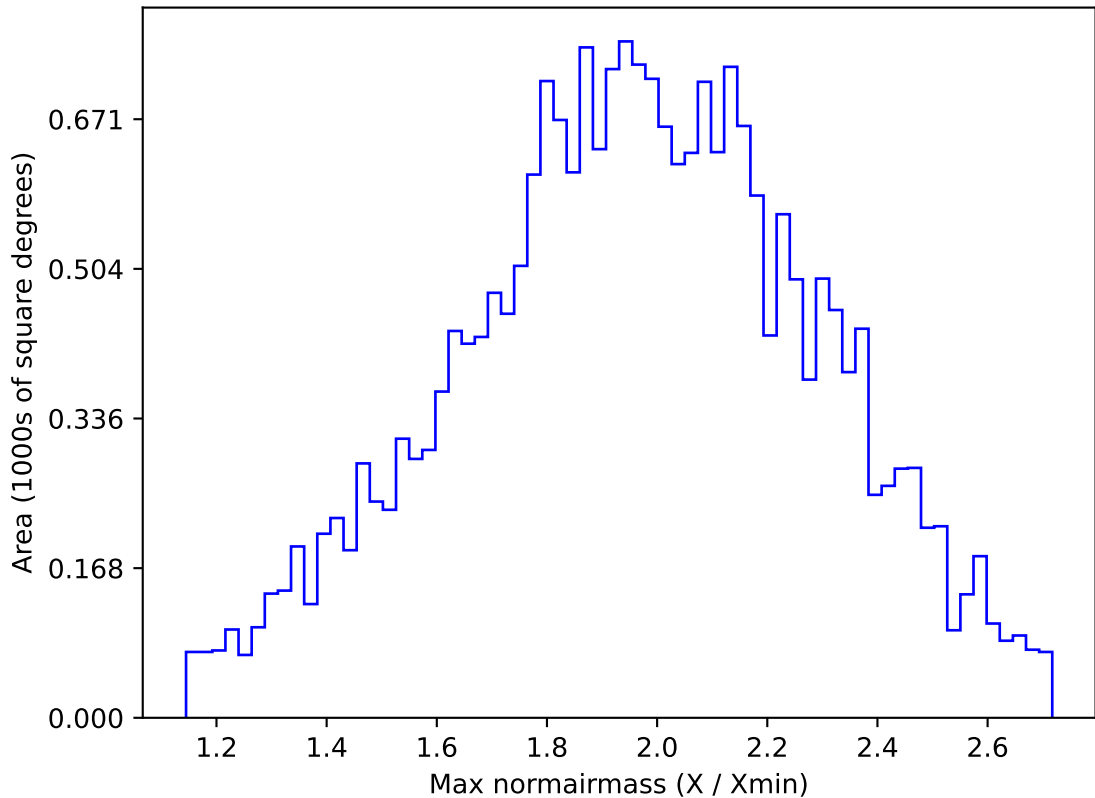
roll_pause_mjdp270_v3.4_10yrs All sky y band: Max normairmass
