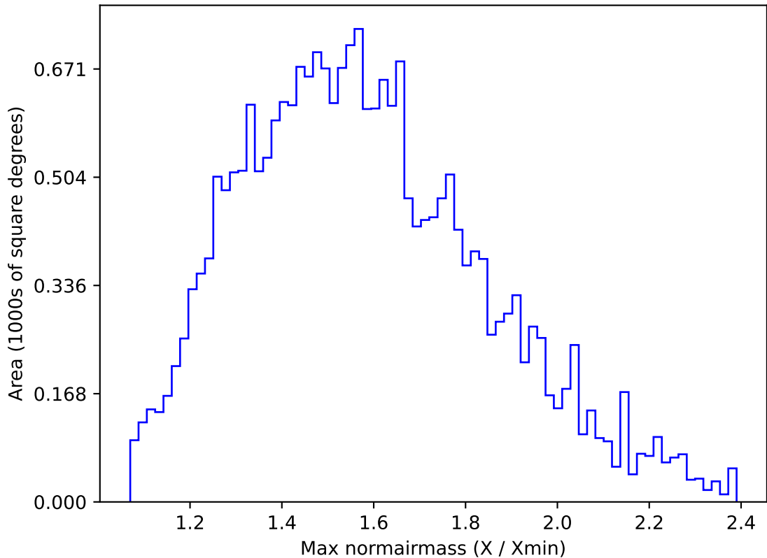
roll_pause_mjdp270_v3.4_10yrs All sky u band: Max normairmass
