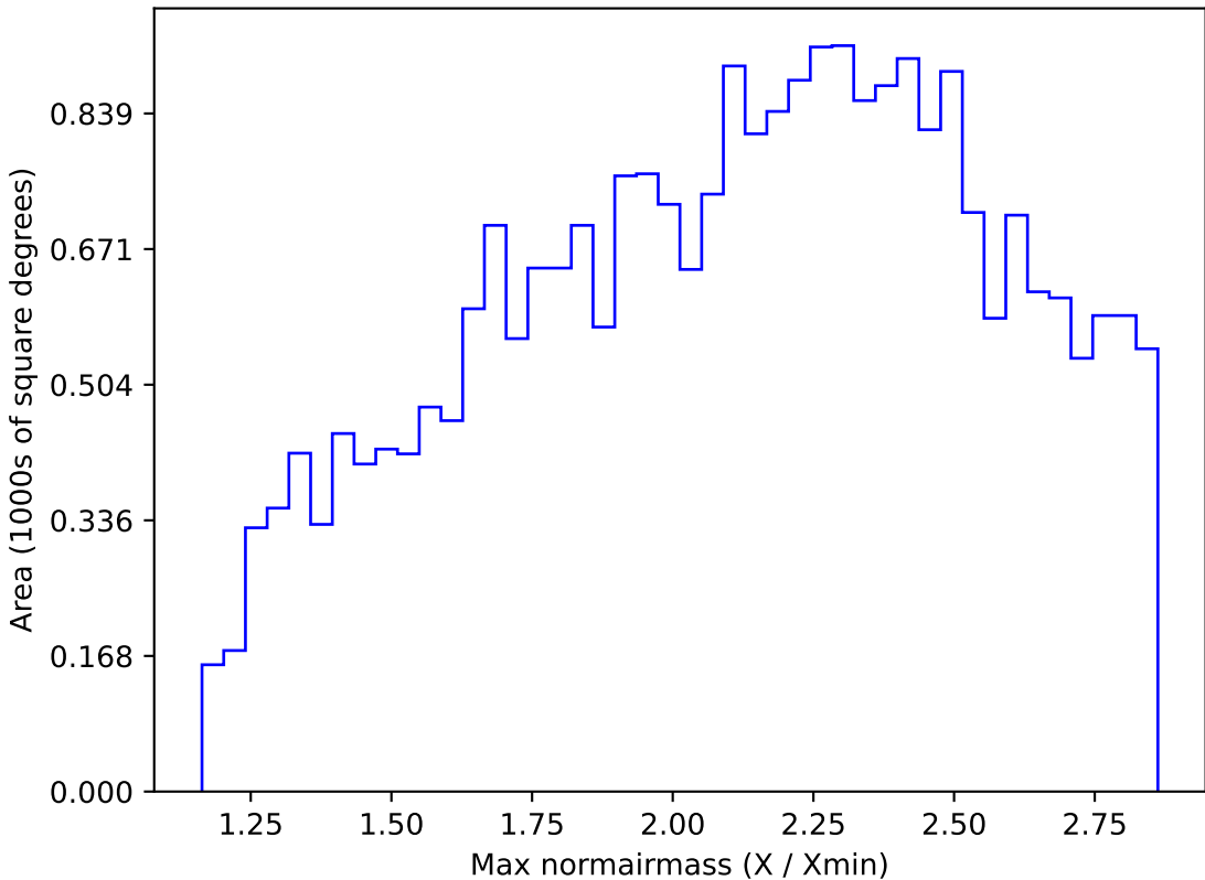
roll_pause_mjdp270_v3.4_10yrs All sky i band: Max normairmass
