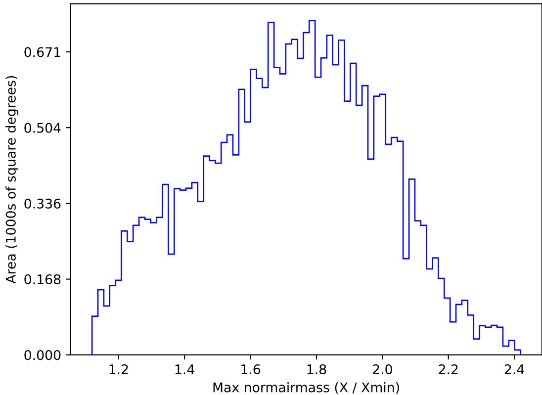
roll_pause_mjdp270_v3.4_10yrs All sky g band: Max normairmass
