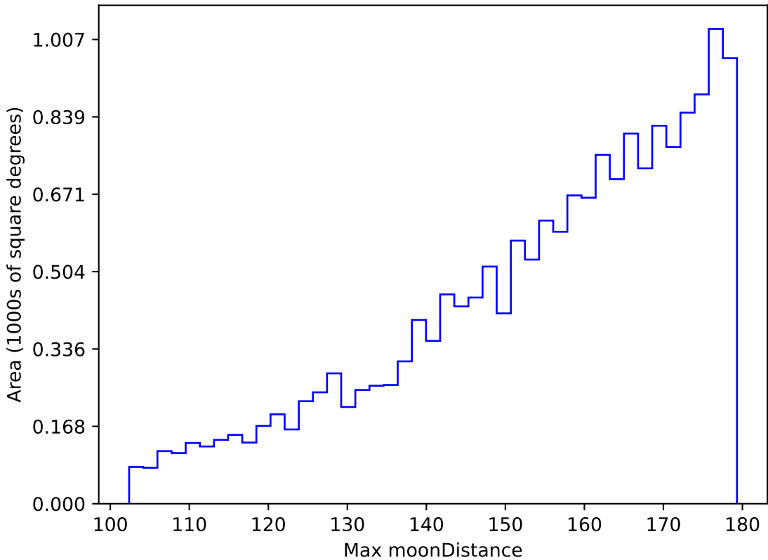
roll_pause_mjdp270_v3.4_10yrs WFD u band: Max moonDistance
