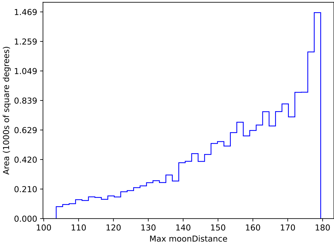
roll_pause_mjdp270_v3.4_10yrs WFD r band: Max moonDistance
