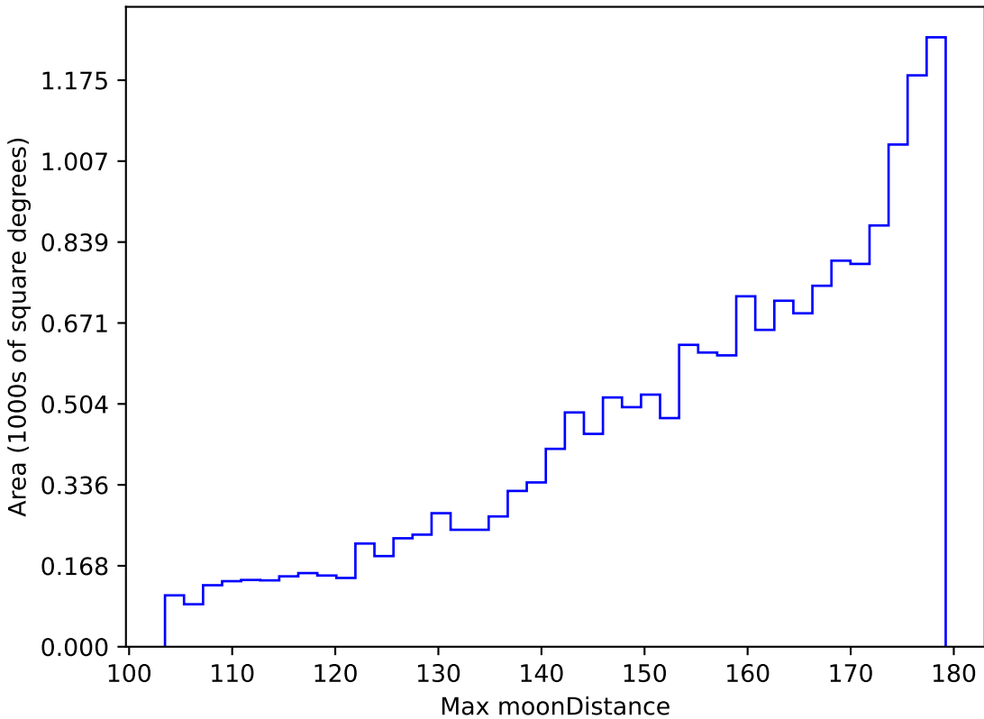
roll_pause_mjdp270_v3.4_10yrs WFD i band: Max moonDistance
