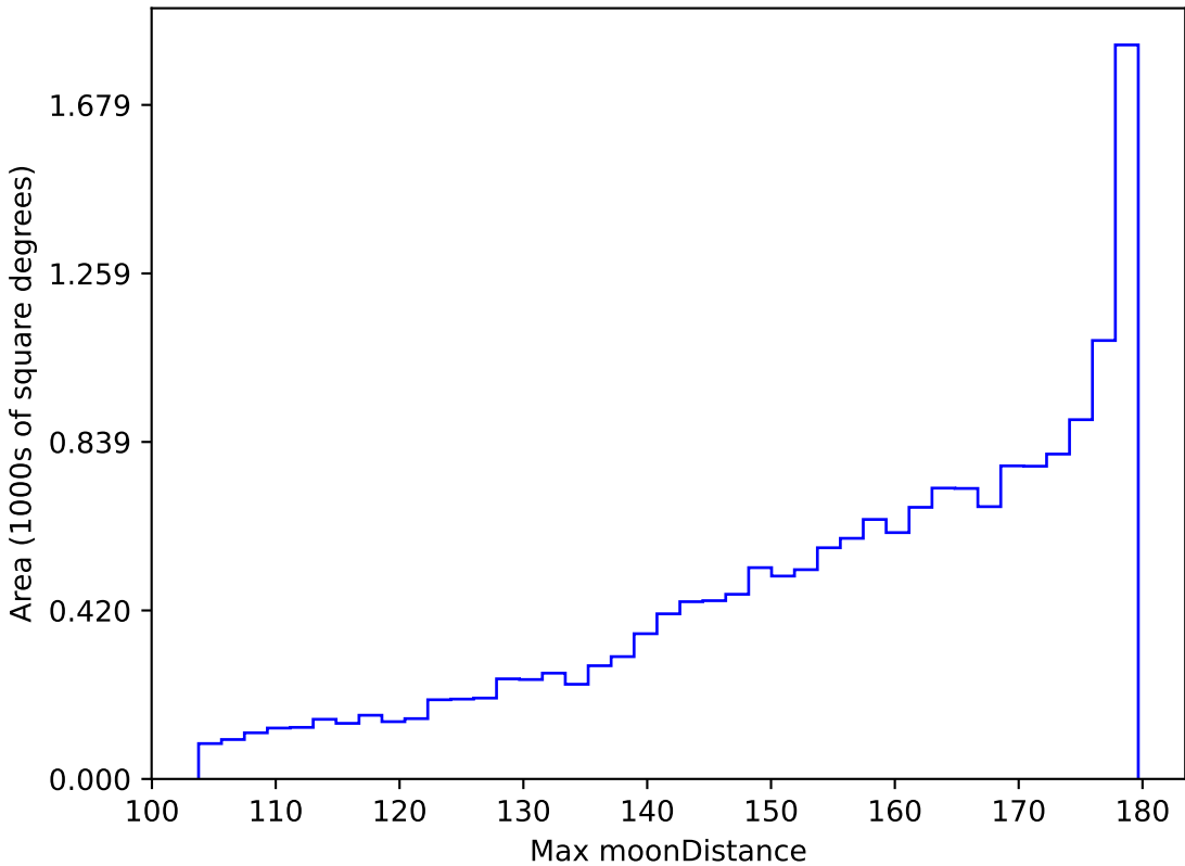
roll_pause_mjdp270_v3.4_10yrs WFD all bands: Max moonDistance
