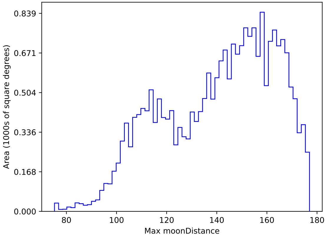
roll_pause_mjdp270_v3.4_10yrs All sky y band: Max moonDistance
