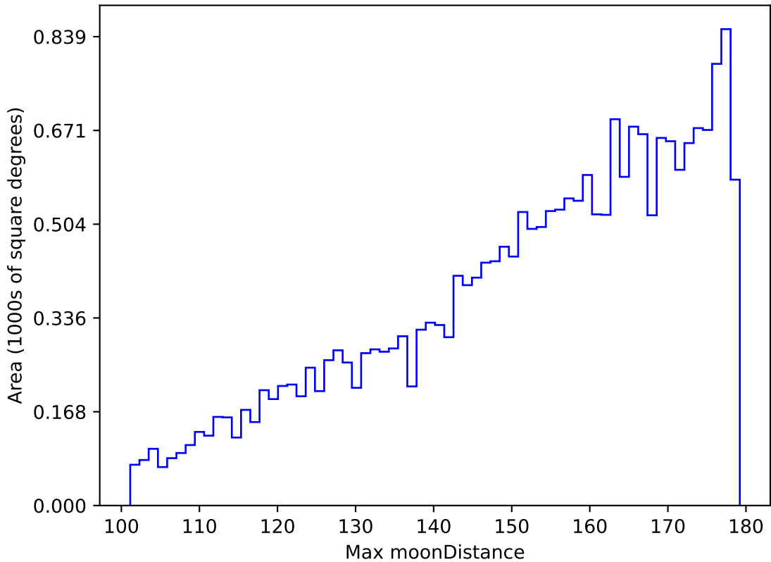
roll_pause_mjdp270_v3.4_10yrs All sky u band: Max moonDistance
