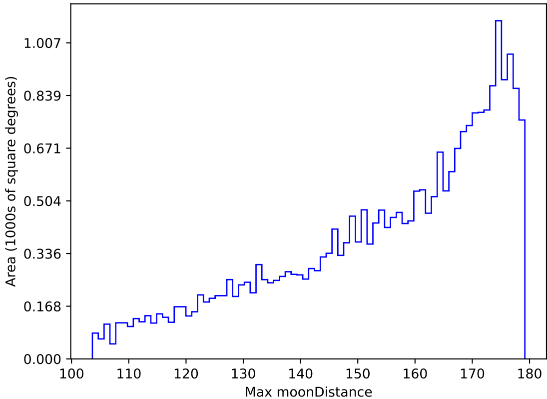
roll_pause_mjdp270_v3.4_10yrs All sky g band: Max moonDistance
