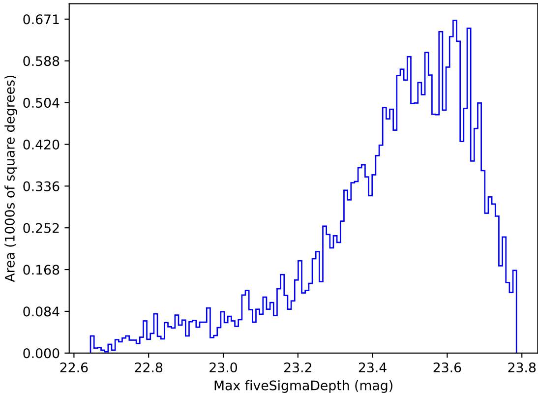
roll_pause_mjdp270_v3.4_10yrs Yr 1 z band: Max fiveSigmaDepth
