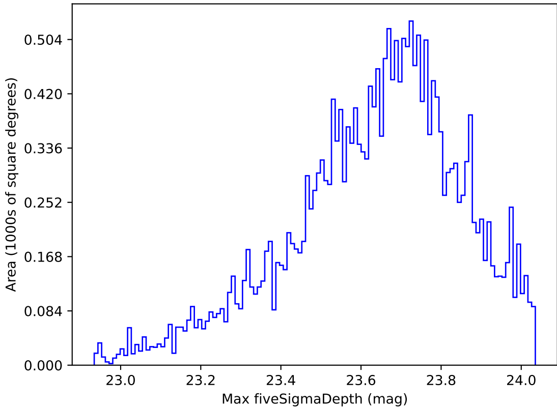
roll_pause_mjdp270_v3.4_10yrs Yr 1 u band: Max fiveSigmaDepth
