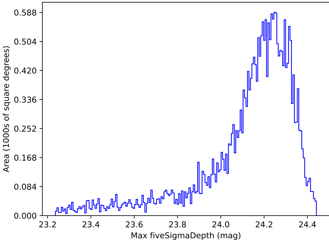
roll_pause_mjdp270_v3.4_10yrs Yr 1 i band: Max fiveSigmaDepth
