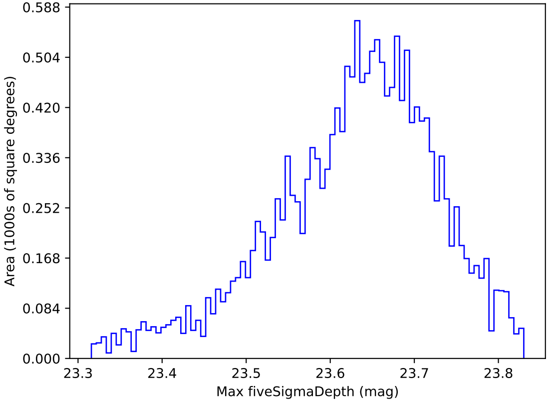
roll_pause_mjdp270_v3.4_10yrs WFD z band: Max fiveSigmaDepth
