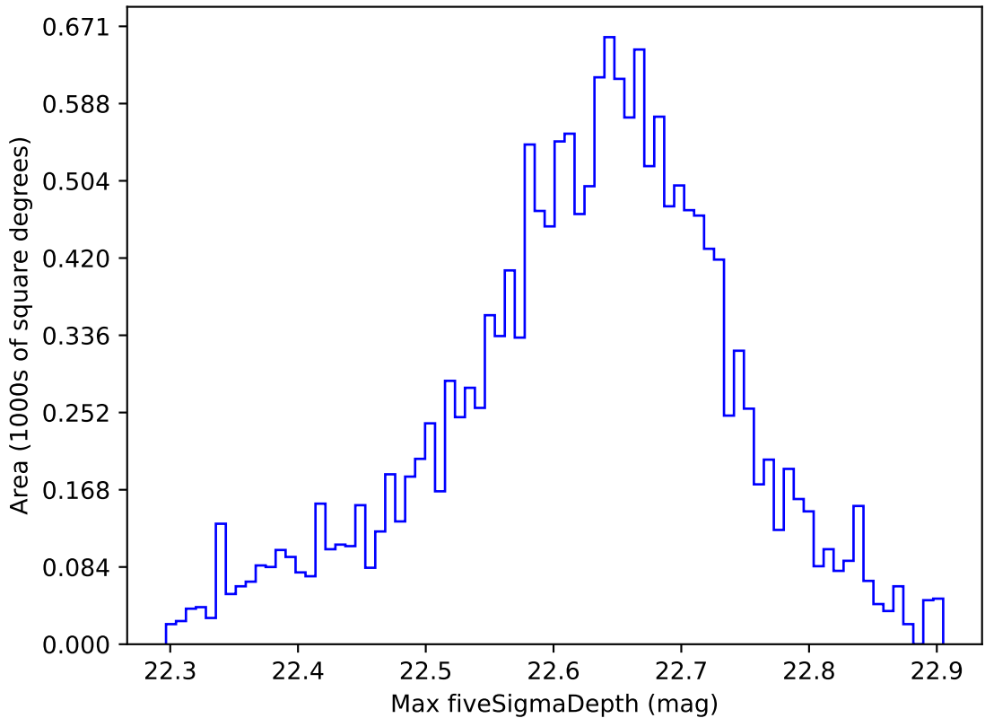
roll_pause_mjdp270_v3.4_10yrs WFD y band: Max fiveSigmaDepth
