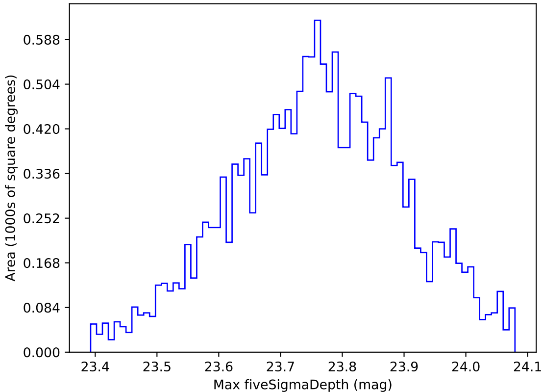
roll_pause_mjdp270_v3.4_10yrs WFD u band: Max fiveSigmaDepth
