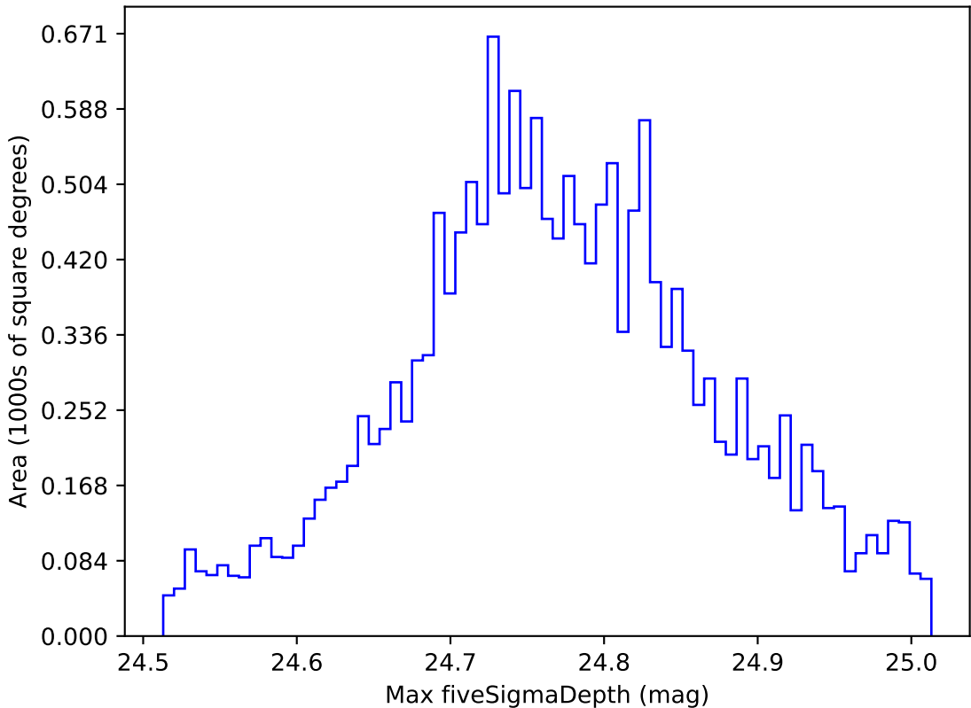
roll_pause_mjdp270_v3.4_10yrs WFD r band: Max fiveSigmaDepth
