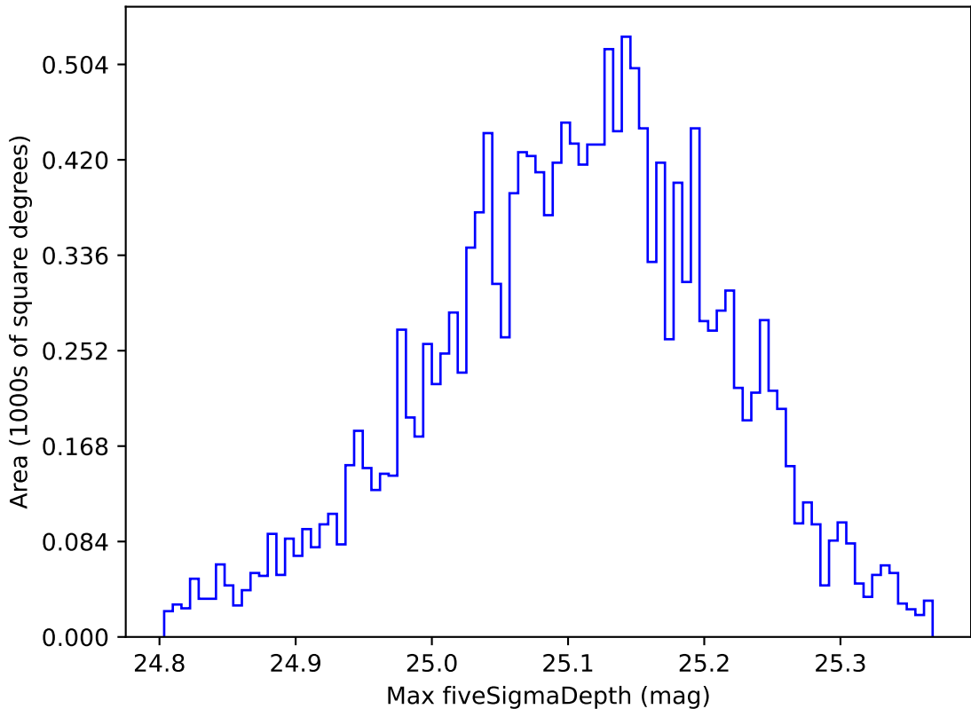
roll_pause_mjdp270_v3.4_10yrs WFD g band: Max fiveSigmaDepth
