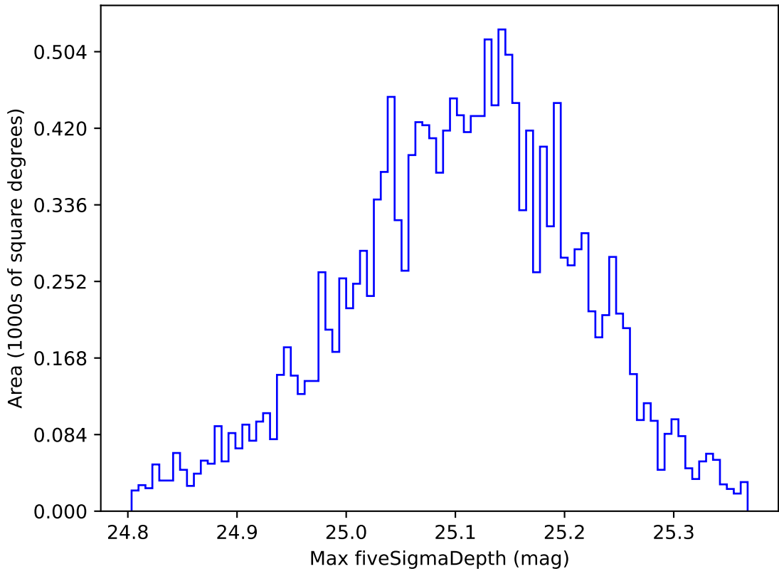
roll_pause_mjdp270_v3.4_10yrs WFD all bands: Max fiveSigmaDepth
