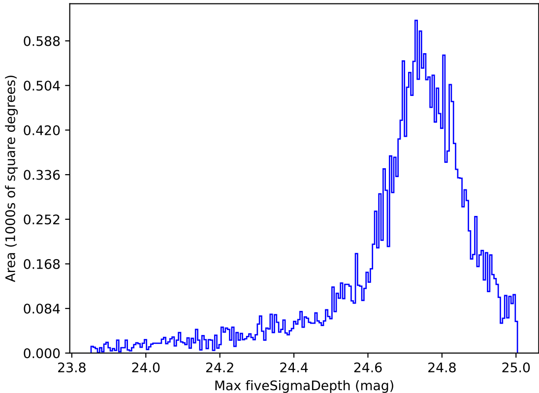
roll_pause_mjdp270_v3.4_10yrs All sky r band: Max fiveSigmaDepth
