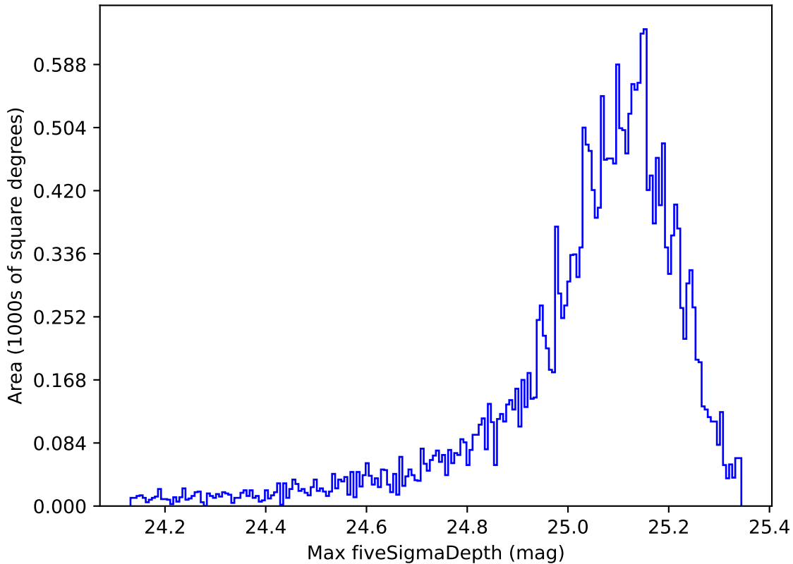
roll_pause_mjdp270_v3.4_10yrs All sky all bands: Max fiveSigmaDepth
