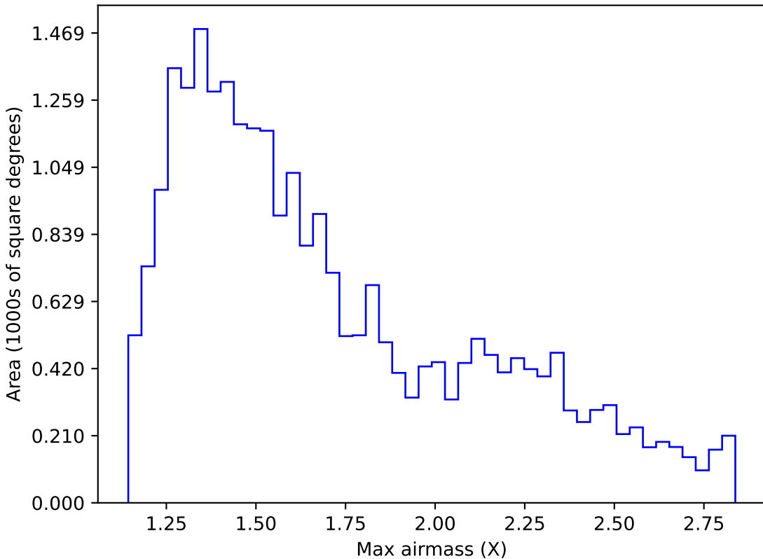
roll_pause_mjdp270_v3.4_10yrs Yr 1 z band: Max airmass
