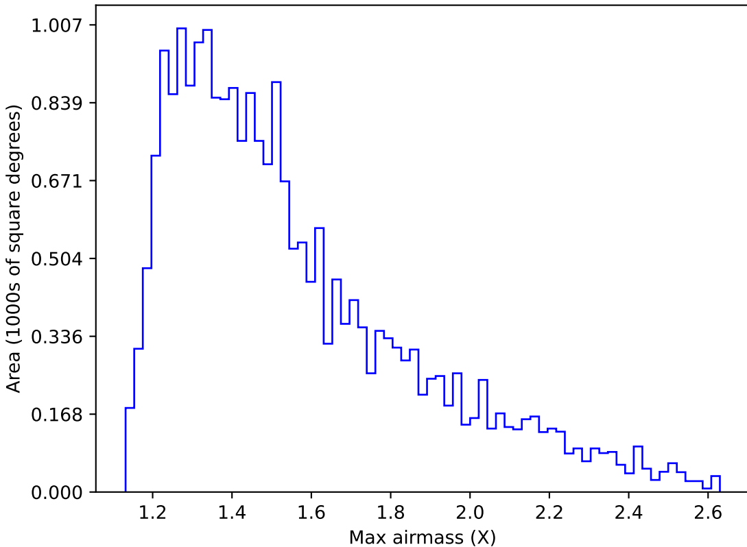
roll_pause_mjdp270_v3.4_10yrs Yr 1 y band: Max airmass
