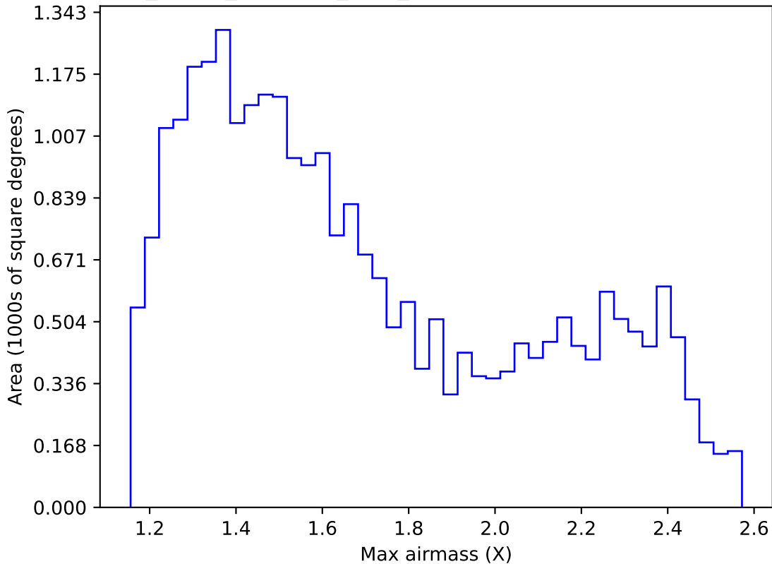
roll_pause_mjdp270_v3.4_10yrs Yr 1 r band: Max airmass
