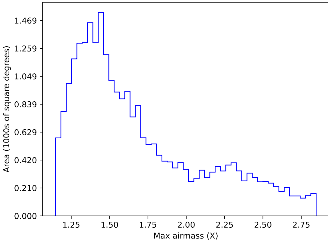
roll_pause_mjdp270_v3.4_10yrs Yr 1 i band: Max airmass
