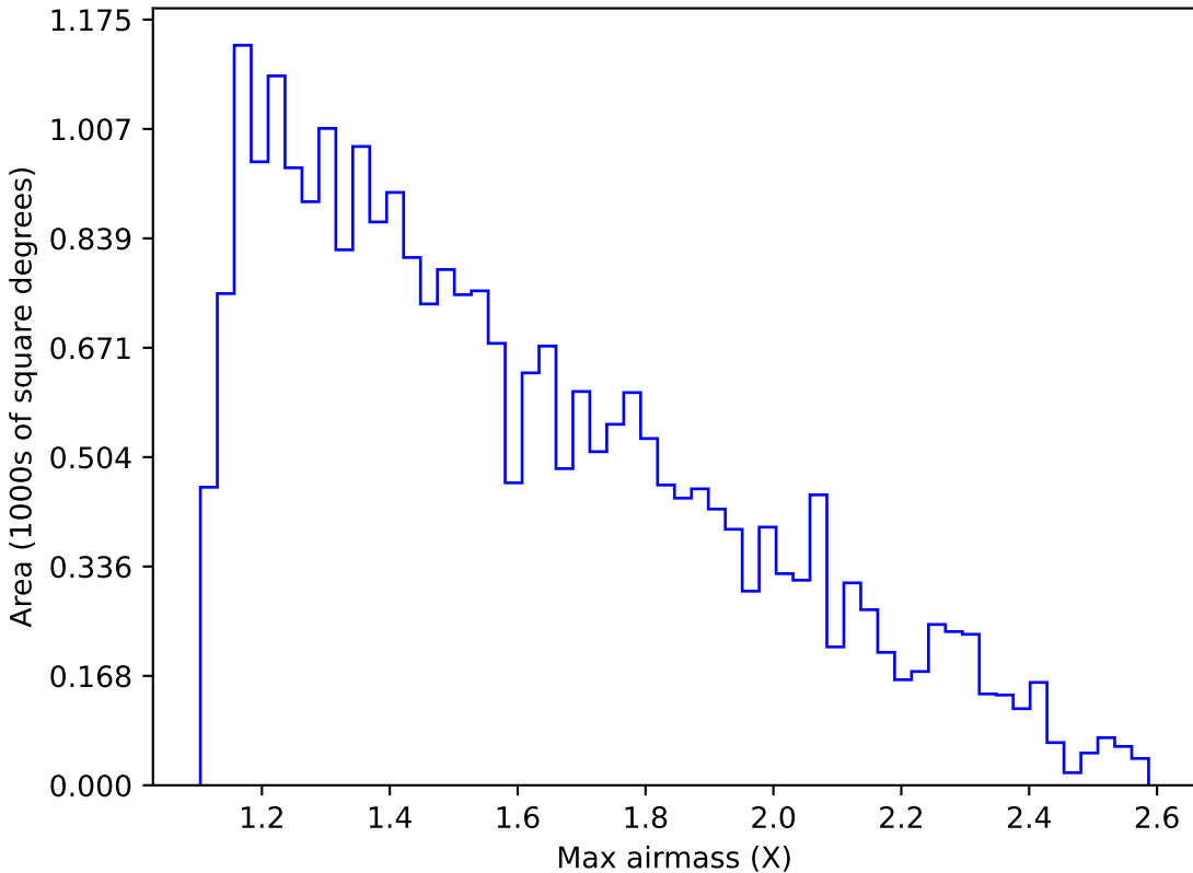
roll_pause_mjdp270_v3.4_10yrs Yr 1 g band: Max airmass
