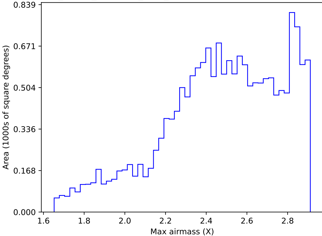
roll_pause_mjdp270_v3.4_10yrs WFD z band: Max airmass
