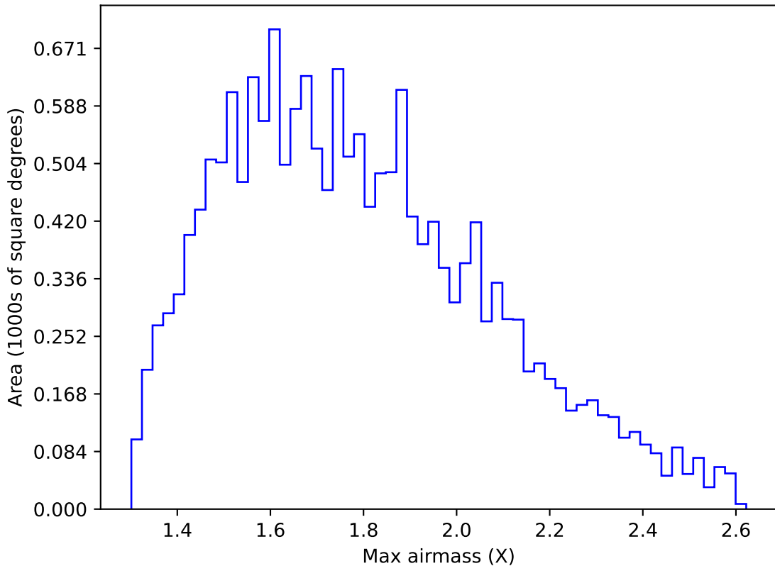
roll_pause_mjdp270_v3.4_10yrs WFD u band: Max airmass
