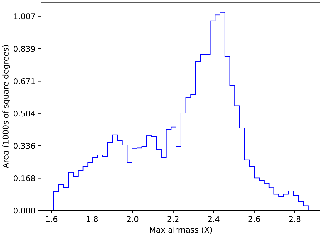
roll_pause_mjdp270_v3.4_10yrs WFD r band: Max airmass
