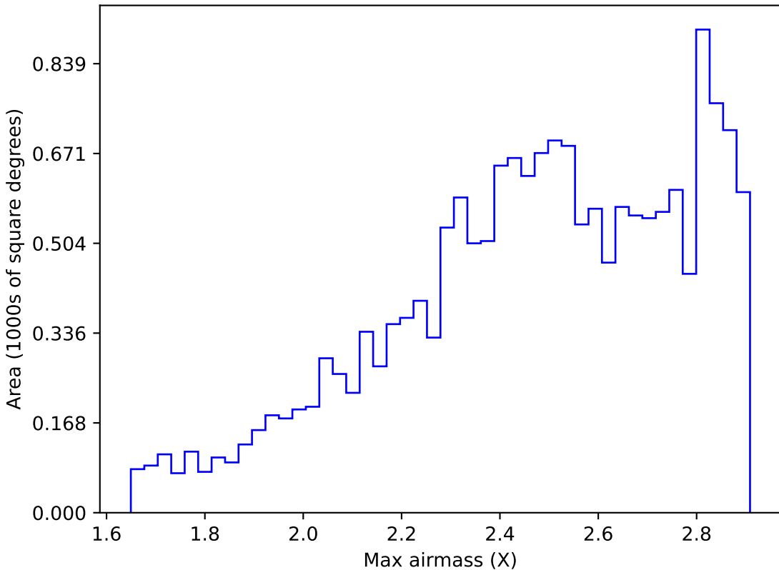
roll_pause_mjdp270_v3.4_10yrs WFD i band: Max airmass
