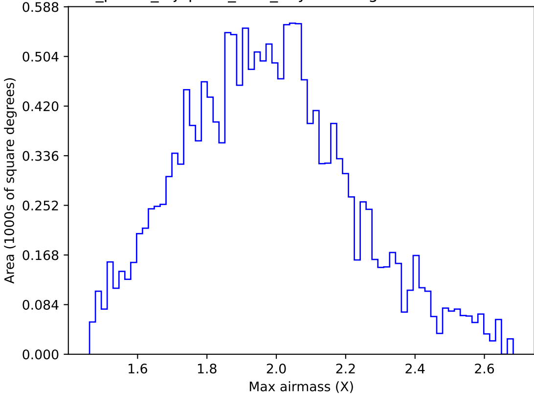
roll_pause_mjdp270_v3.4_10yrs WFD g band: Max airmass
