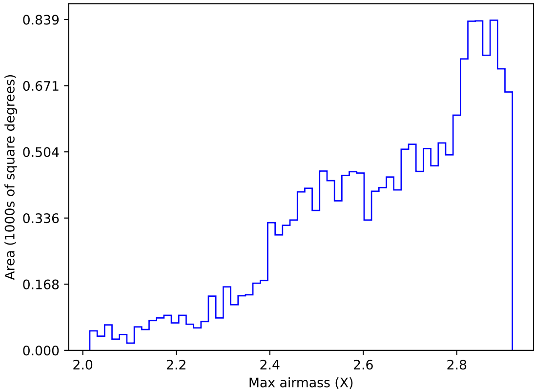
roll_pause_mjdp270_v3.4_10yrs WFD all bands: Max airmass
