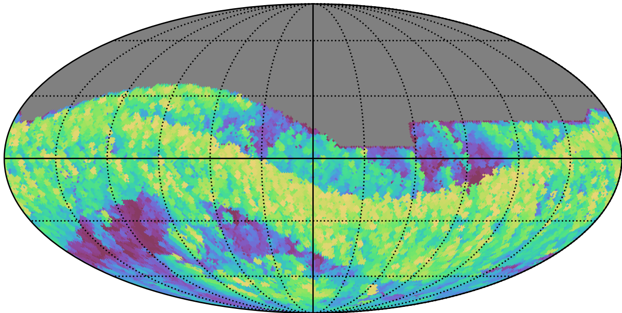
roll_pause_mjdp270_v3.4_10yrs All sky z band: Max airmass
