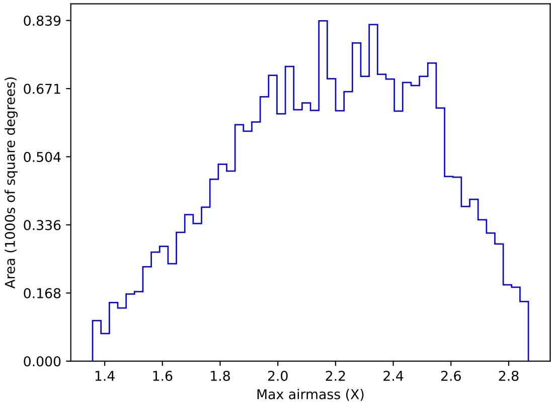
roll_pause_mjdp270_v3.4_10yrs All sky y band: Max airmass
