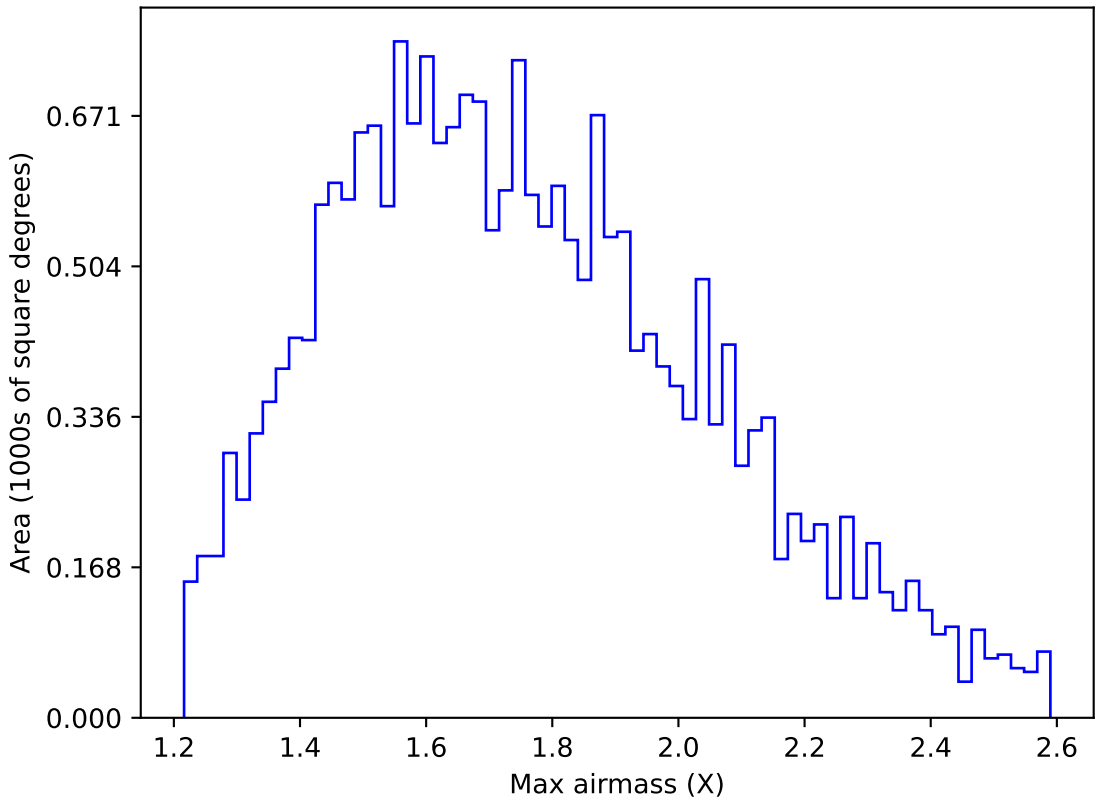
roll_pause_mjdp270_v3.4_10yrs All sky u band: Max airmass
