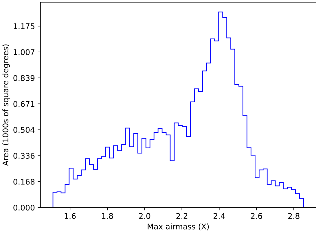
roll_pause_mjdp270_v3.4_10yrs All sky r band: Max airmass
