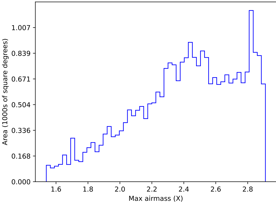
roll_pause_mjdp270_v3.4_10yrs All sky i band: Max airmass
