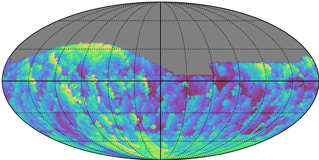
roll_pause_mjdp270_v3.4_10yrs All sky g band: Max airmass
