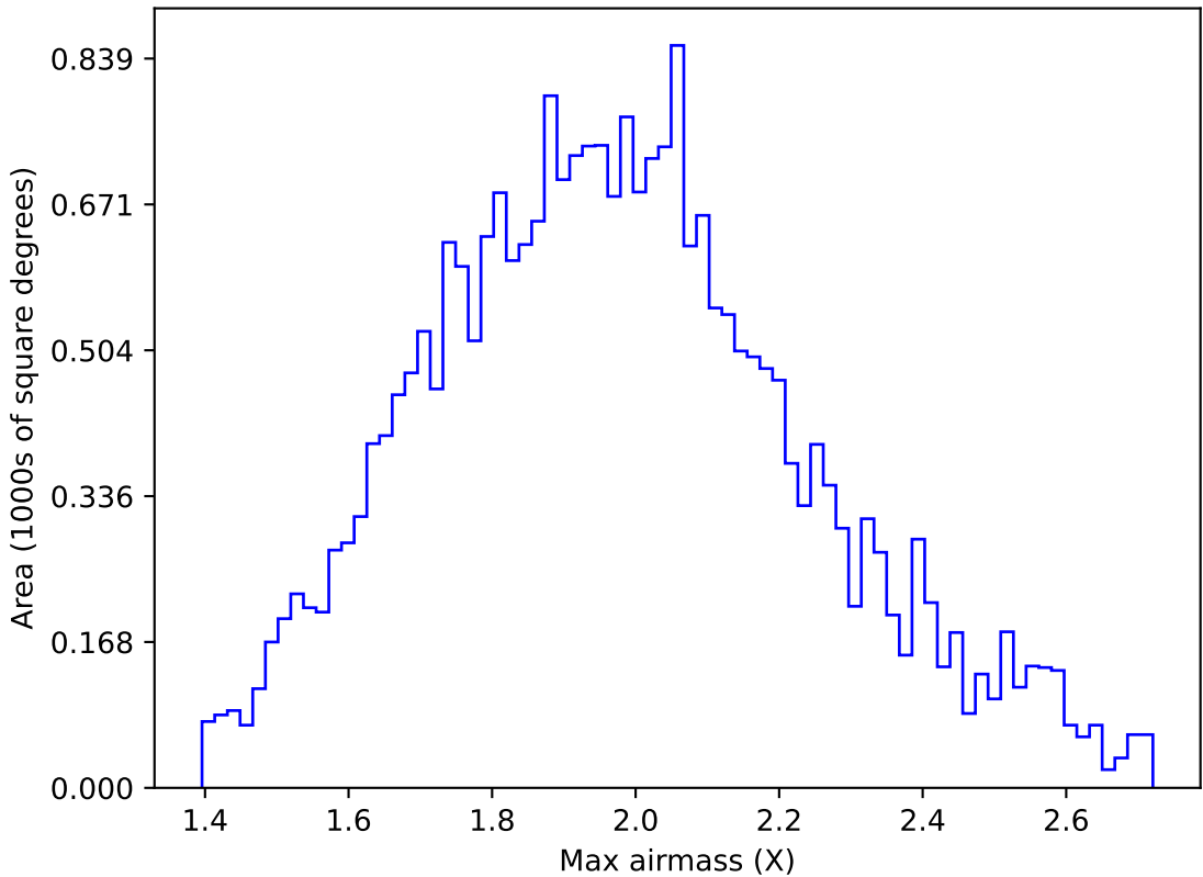
roll_pause_mjdp270_v3.4_10yrs All sky g band: Max airmass
