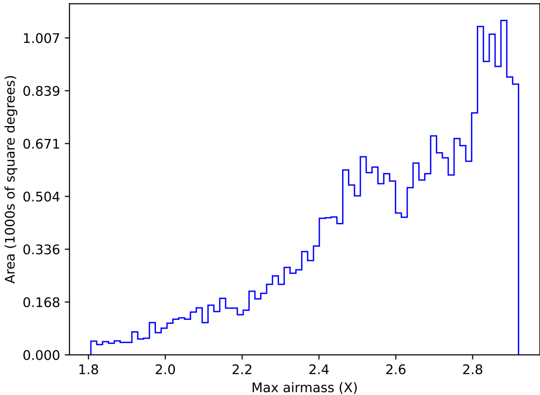
roll_pause_mjdp270_v3.4_10yrs All sky all bands: Max airmass
