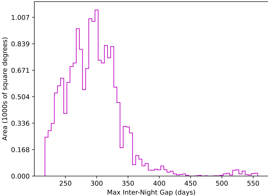
roll_pause_mjdp270_v3.4_10yrs WFD z band: Max Inter-Night Gap
