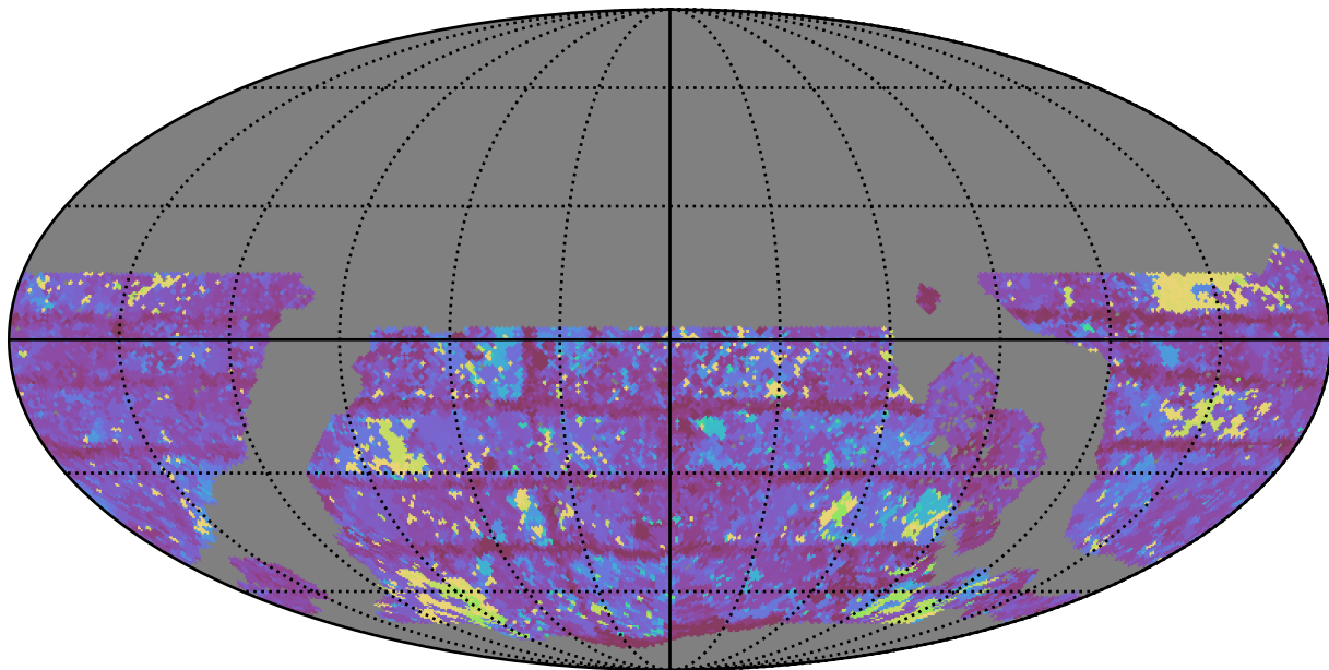
roll_pause_mjdp270_v3.4_10yrs WFD y band: Max Inter-Night Gap
