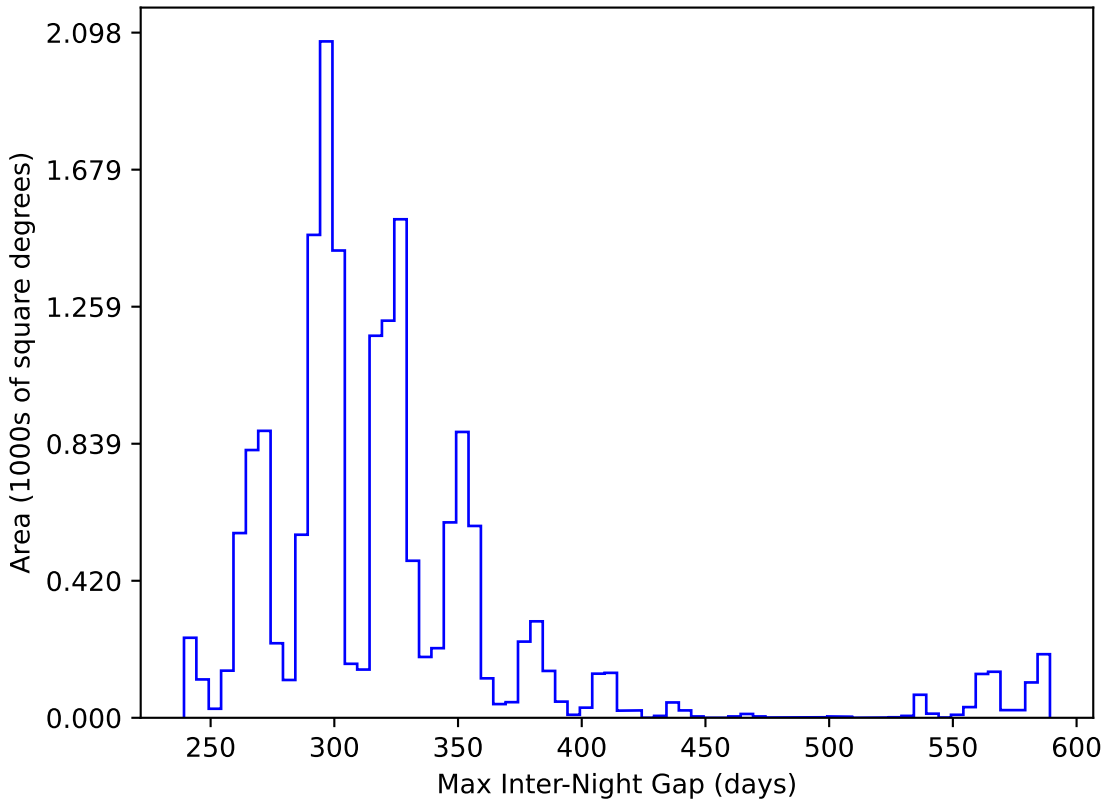
roll_pause_mjdp270_v3.4_10yrs WFD y band: Max Inter-Night Gap
