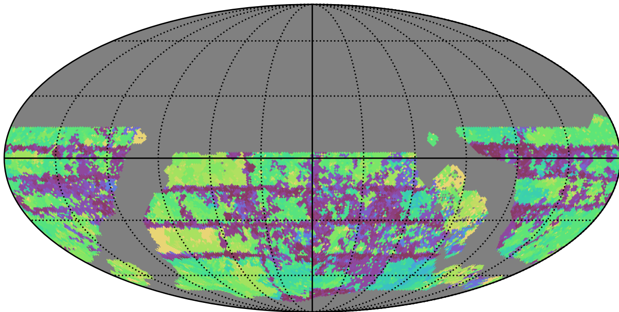
roll_pause_mjdp270_v3.4_10yrs WFD u band: Max Inter-Night Gap
